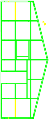
FRONT WALL FRAMING
