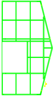
REAR WALL FRAMING
