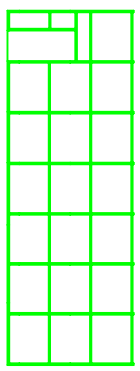
LEFT SIDE WALL FRAMING
