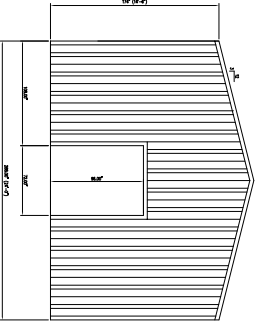
BACK ELEVATION
