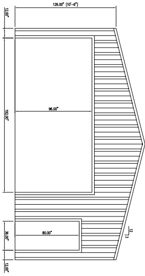
FRONT WALL ELEVATION
