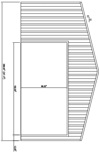
BACK WALL ELEVATION
