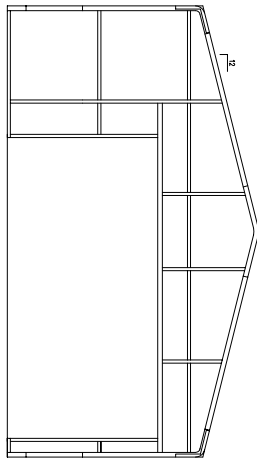
BACK WALL FRAMING
