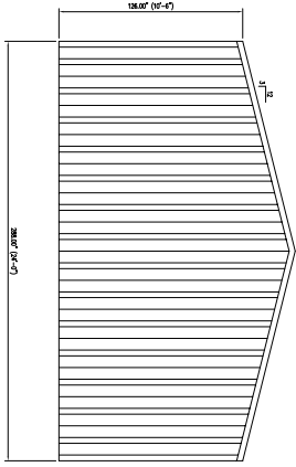
TYPICAL FRONT & BACK ELEVATION
