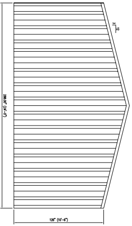
TYPICAL FRONT & BACK ELEVATION
