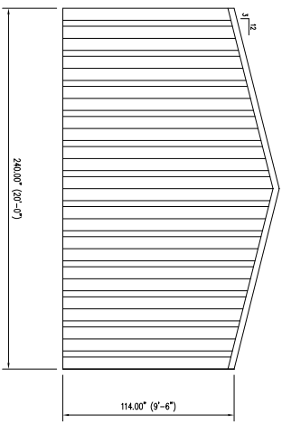
TYPICAL FRONT & BACK ELEVATION
