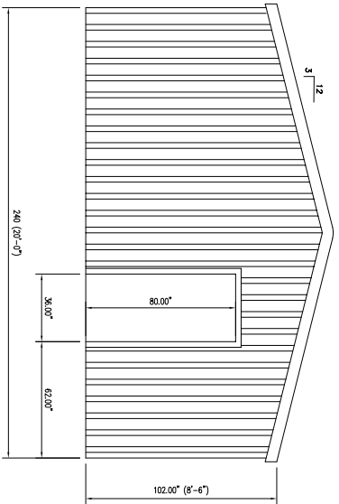
BACK ELEVATION
