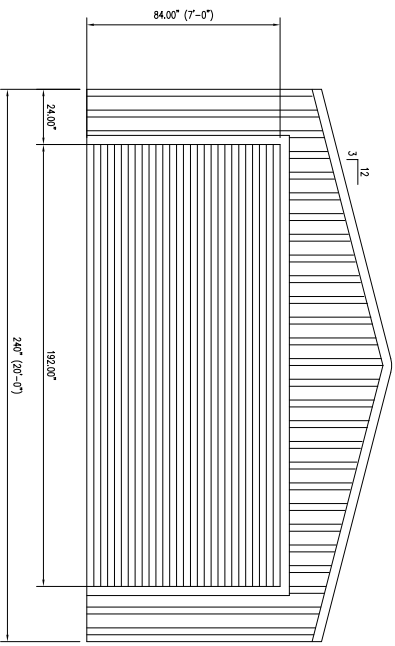
FRONT ELEVATION
