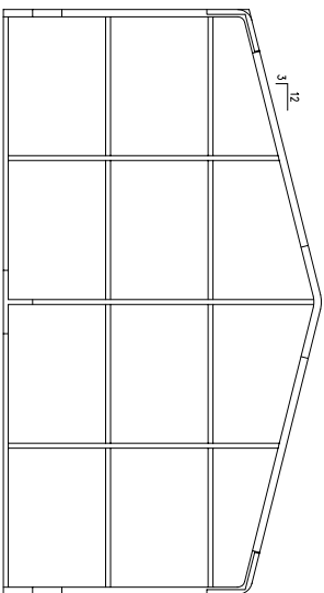
BACK WALL FRAMING
