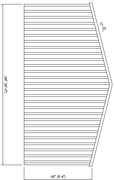
BACK ELEVATION
